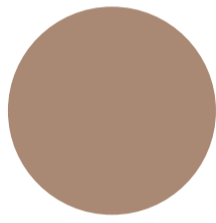
Copper
