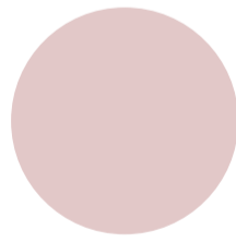
Quartz
